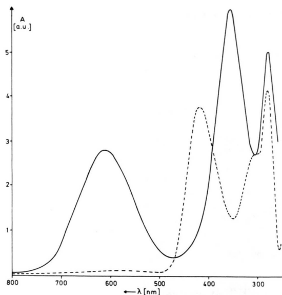
Fig. 1. Absorption spectra of denatured phycocyanin (48 \mu M) in phosphate buffer (50 mM, pH 7.5) containing urea (8 M) (—), and of the same solution after addition of \text{NaBH}_4 in the same solvent (---). The borohydride was added in two equal portions corresponding to a nominal final concentration of 24 mM, at times 0 and 30 min, the spectrum was recorded at t = 60 min.
