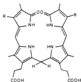
6a R = C_2H_3 6b R = C_2H_5
